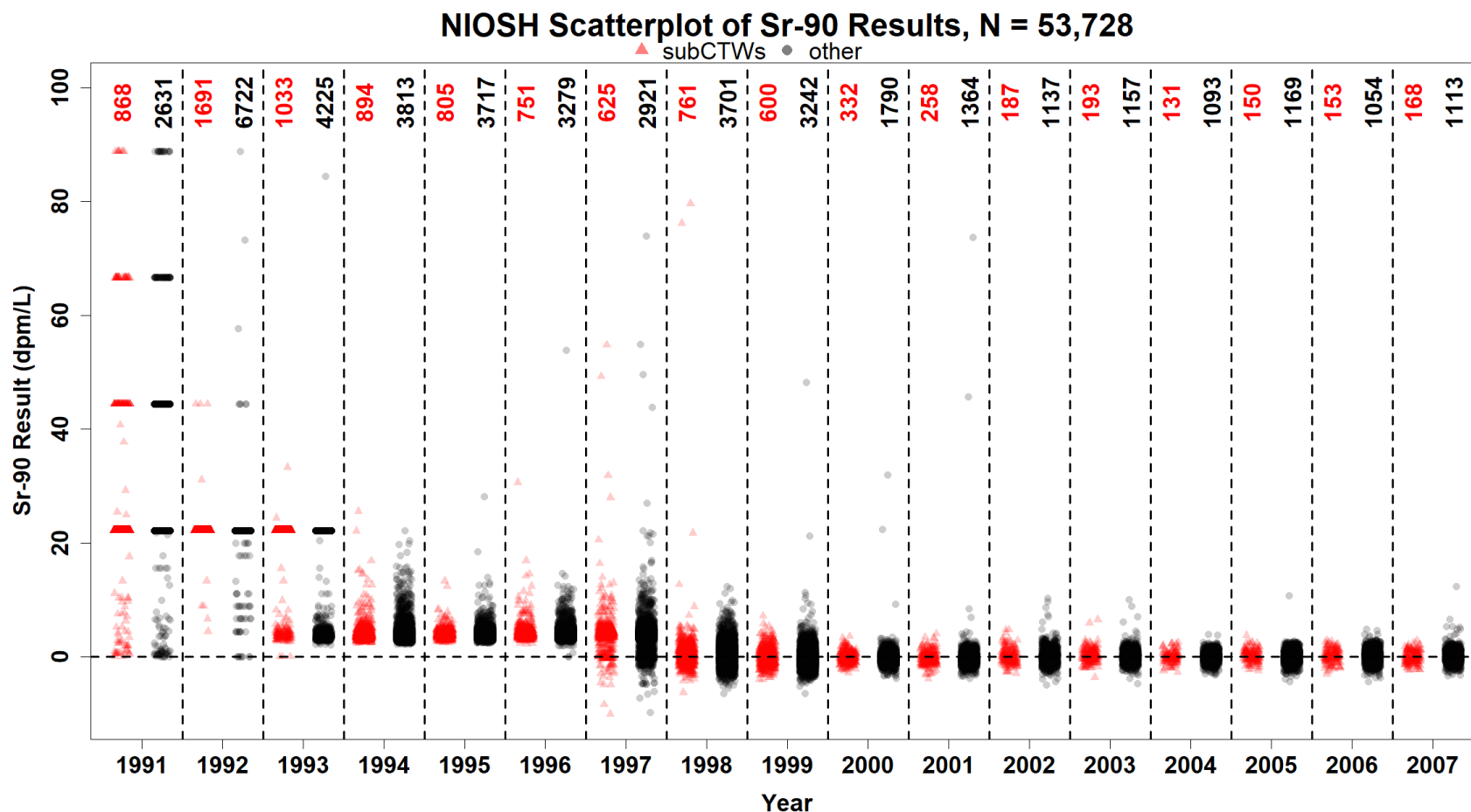
Figure C-22: Scatterplot Using SC&A Definition of Subcontractors (red, left) and Primes (black, right) Strontium Bioassay Data with a Zoomed Y-Axis.
