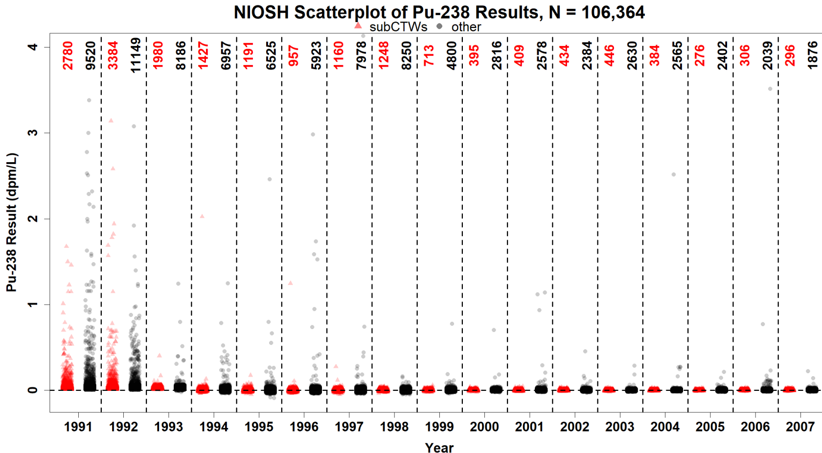
Figure 10: Scatterplot of subCTW (red, left) and Other Worker (black, right) Pu-238 Bioassay Data with a Zoomed Y-Axis.
