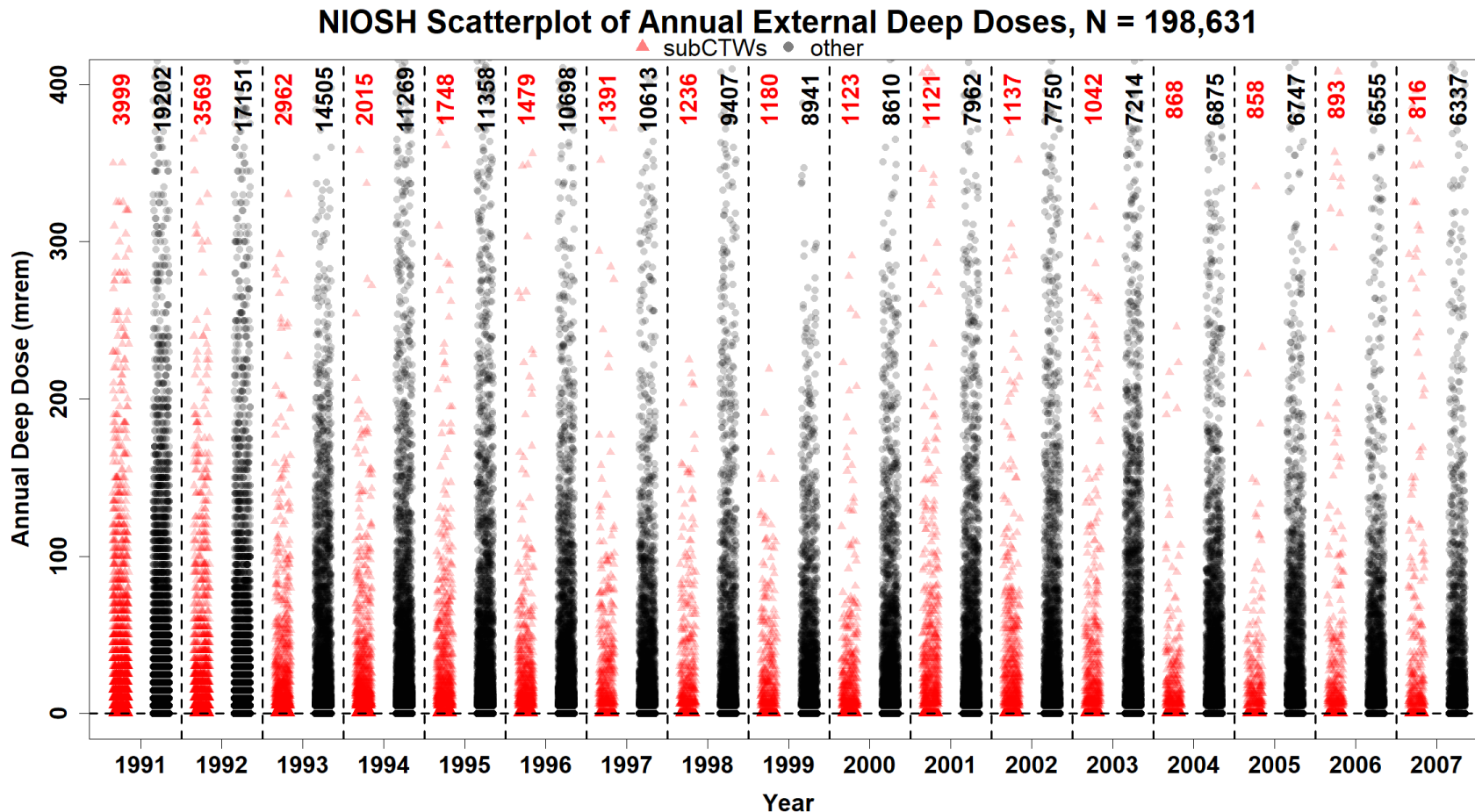
Figure 4: Scatterplot of subCTW (red, left) and Other Worker (black, right) Annual Deep Doses with a Zoomed Y-Axis.
