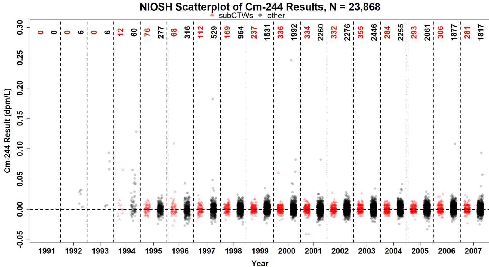
Figure C-15: Scatterplot Using SC&A Definition of Subcontractors (red, left) and Primes (black, right) Curium Bioassay Data.
