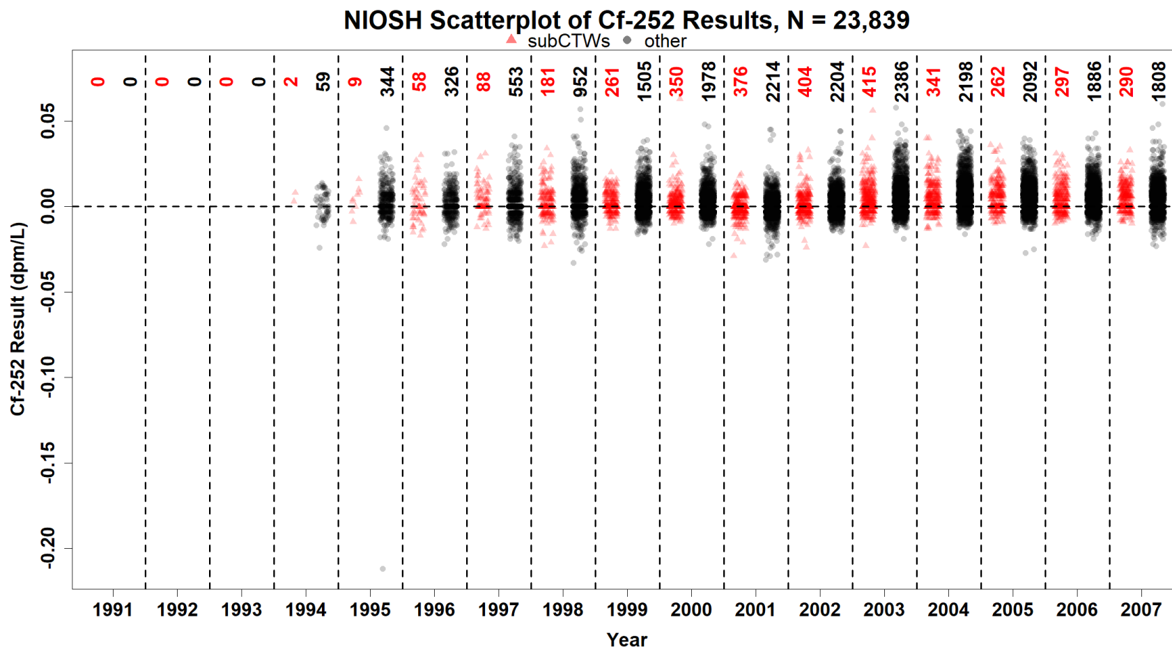
Figure 16: Scatterplot of subCTW (red, left) and Other Worker (black, right) Californium Bioassay Data.
