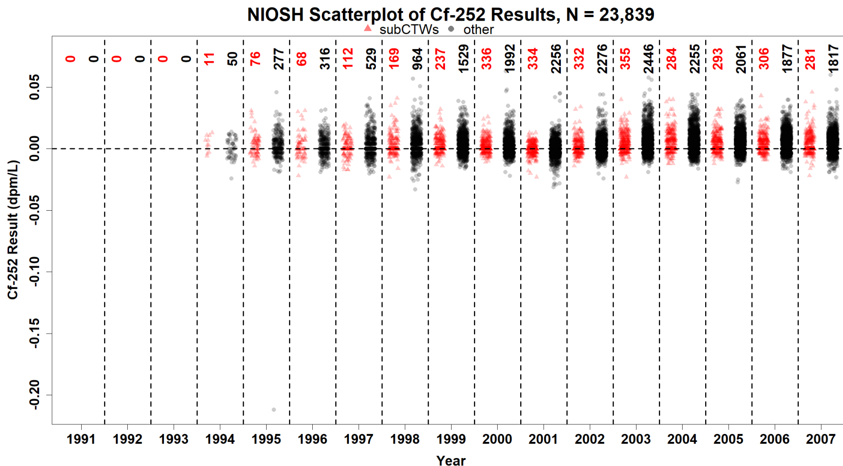
Figure C-16: Scatterplot Using SC&A Definition of Subcontractors (red, left) and Primes (black, right) Californium Bioassay Data.
