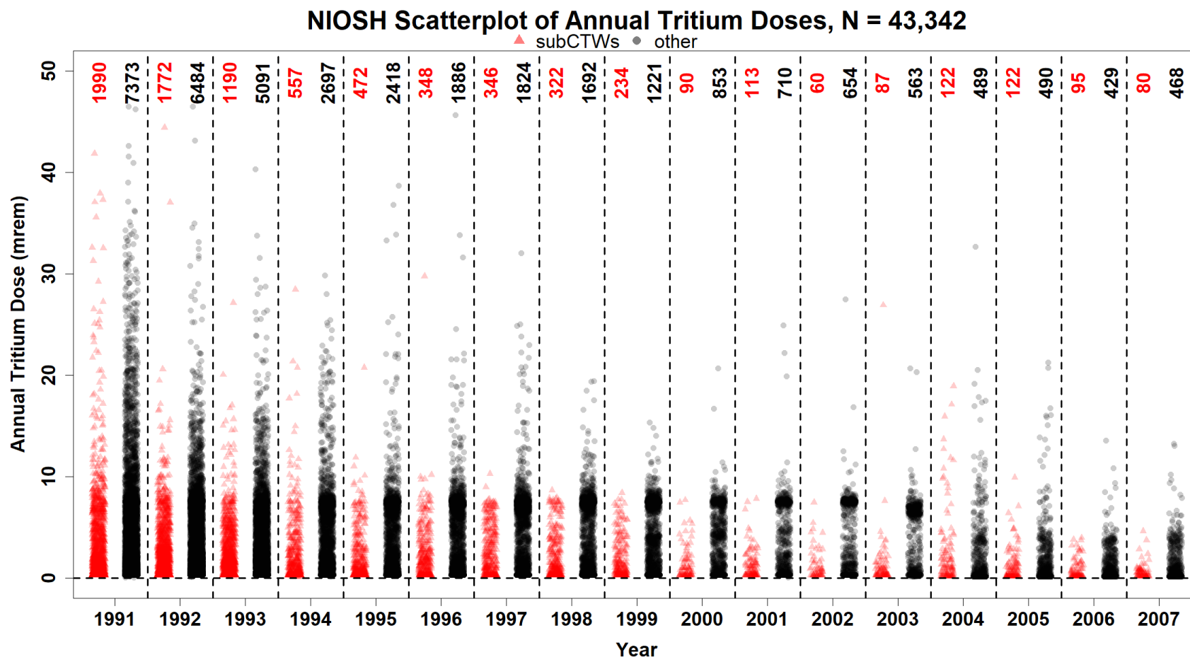
Figure 8: Scatterplot of subCTW (red, left) and Other Worker (black, right) Annual Tritium Doses with a Zoomed Y-Axis.
