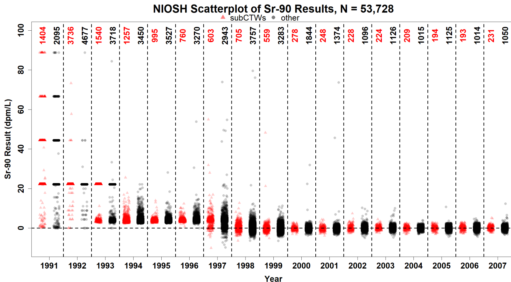
Figure 22: Scatterplot of subCTW (red, left) and Other Worker (black, right) Strontium Bioassay Data with a Zoomed Y-Axis.
