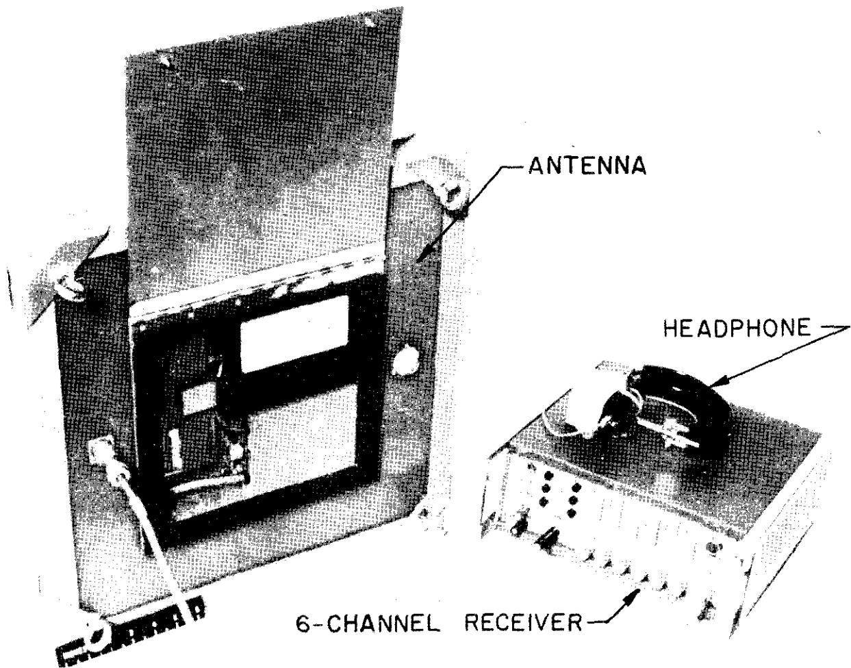
FIGURE 12. - Helicopter receiver.
