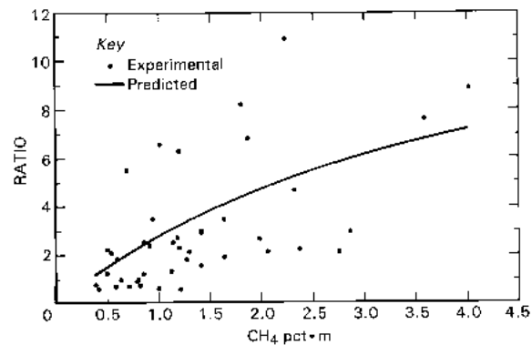
Figure 5.—RATIO versus pct CH 4 •m for 12 experiments.
