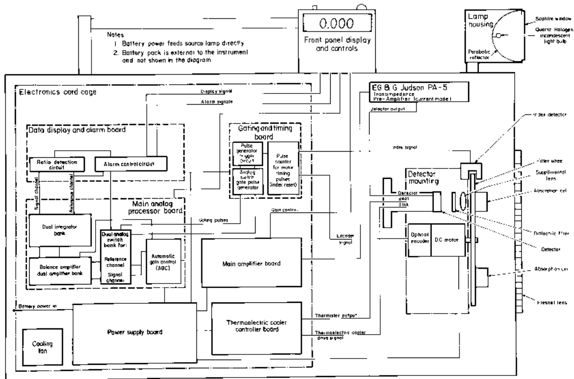
Figure 2.—Block diagram of remote optical methanometer (ROM).
