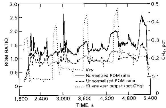
Figure 4.—Measured CH 4 concentration, ROM output signal RATIO, and calculated ROM RATIO.
