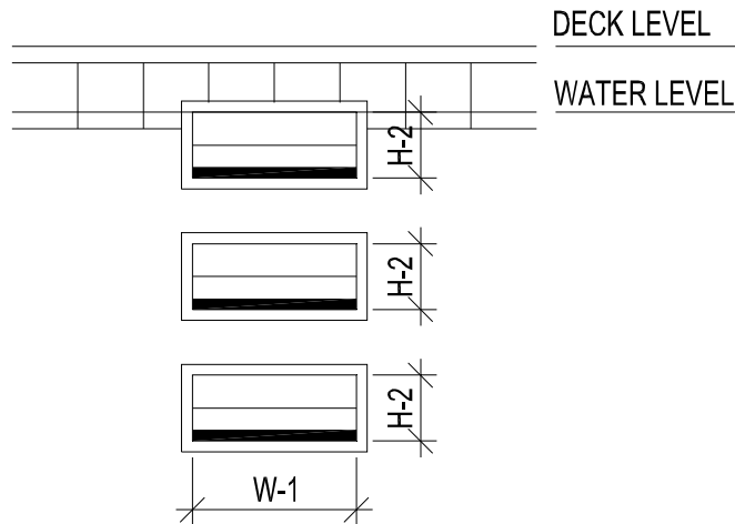
Figure 4.5.7.4.2: Recessed Step Dimensions
