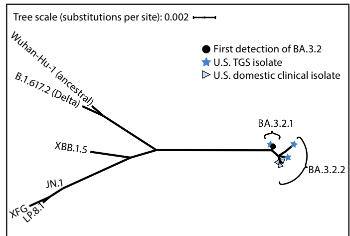
FIGURE 1. Phylogenetic tree* of the SARS-CoV-2 spike glycoprotein gene from selected U.S. † and global § BA.3.2 isolates ¶ and reference strains — 2020–2026
