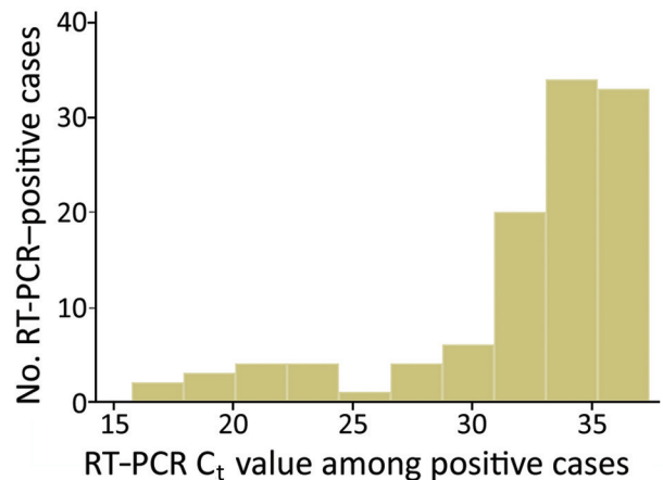
Figure 2. Distribution of real-time RT-PCR C_t values among craft and manual workers identified as real-time RT-PCR positive for severe acute respiratory syndrome coronavirus 2, Qatar. C_t , cycle threshold; RT-PCR, real-time reverse transcription PCR.
