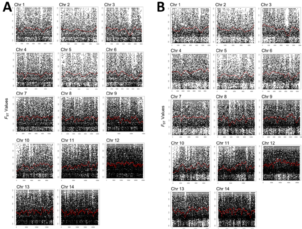
Appendix 1 Figure 2. Genomewide plots of F_{ST} values of allele frequency divergence for all individual SNPs, for comparisons between the Plasmodium knowlesi population in Peninsular Malaysia (cluster 3) and each of the two genetic populations in Malaysian Borneo (clusters 1 and 2). A. cluster 3 versus cluster 1. B. Cluster 3 versus cluster 2. Comparison between P. knowlesi cluster 1 and 2 is not shown as this was published previously (Divis PCS, Duffy CW, Kadir KA, Singh B, Conway DJ. Genomewide mosaicism in divergence between zoonotic malaria parasite subpopulations with separate sympatric transmission cycles. Mol Ecol. 2018;2:860–70). F_{ST} values shown for all individual SNPs with MAF >10%, comparing between P. knowlesi cluster 3 in Peninsular Malaysia and cluster 2 in Malaysian Borneo. In red are shown the means for overlapping windows of 500 SNPs (step size of 250 SNPs along chromosomes).
