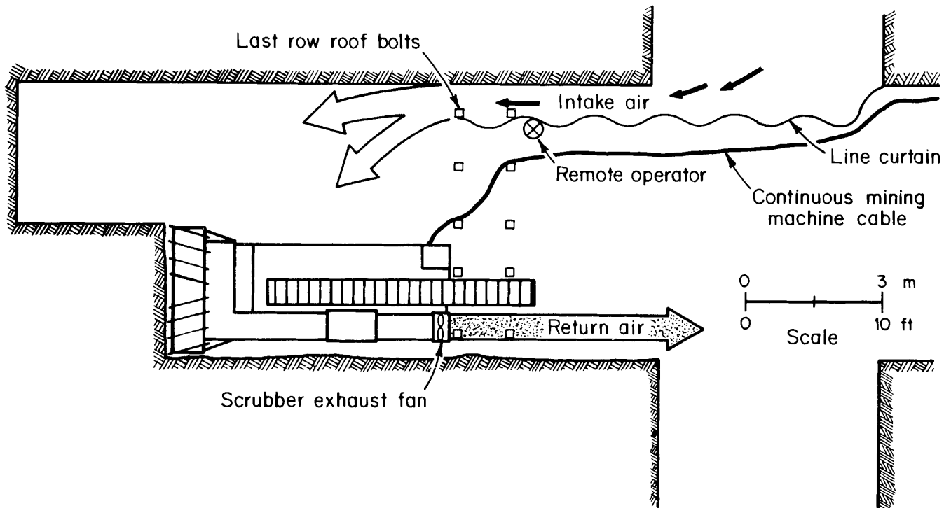
Figure 1.—Diagram of deep-cut mining method.
