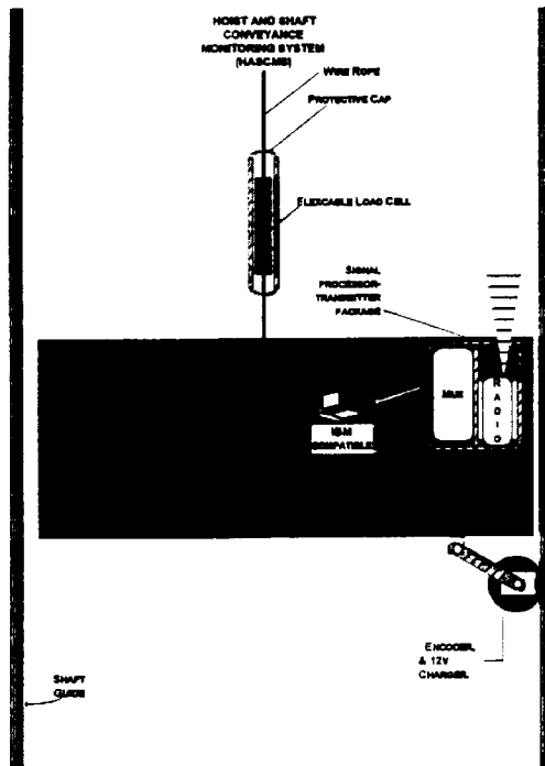
Figure 8. Hoist and shaft conveyance monitoring system.
