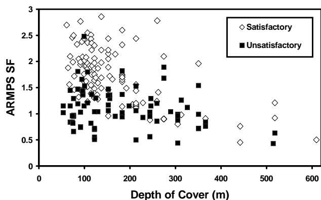
Figure 6. The ARMPS case history data base.
