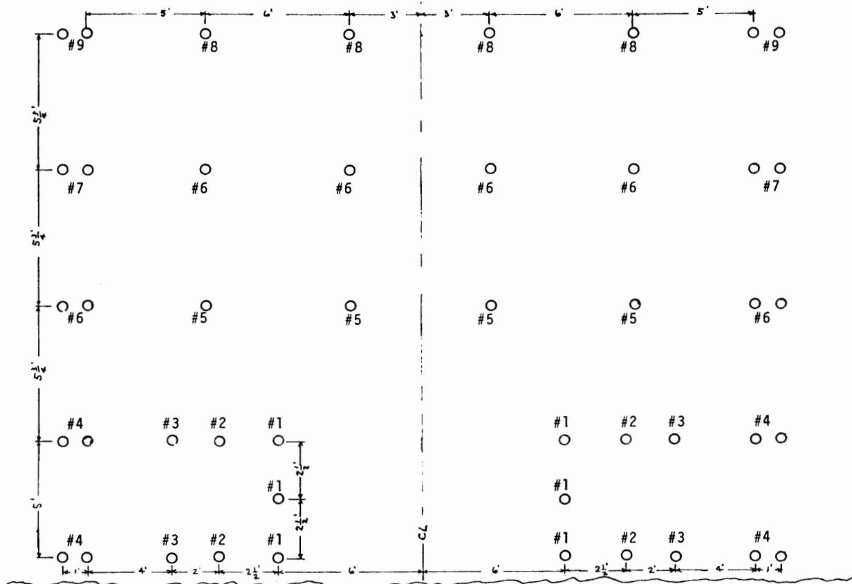
FIGURE 4.1 PATTERN OF HOLES DRILLED IN LIMESTONE FACE FOR BLASTING CAPS USED FOR DEMONSTRATING SAFE RADIO OPERATION OF MOBILE AND PORTABLE UHF RADIOS IN THE VICINITY OF ELECTRIC BLASTING CAPS AND ASSOCIATED WIRING.
