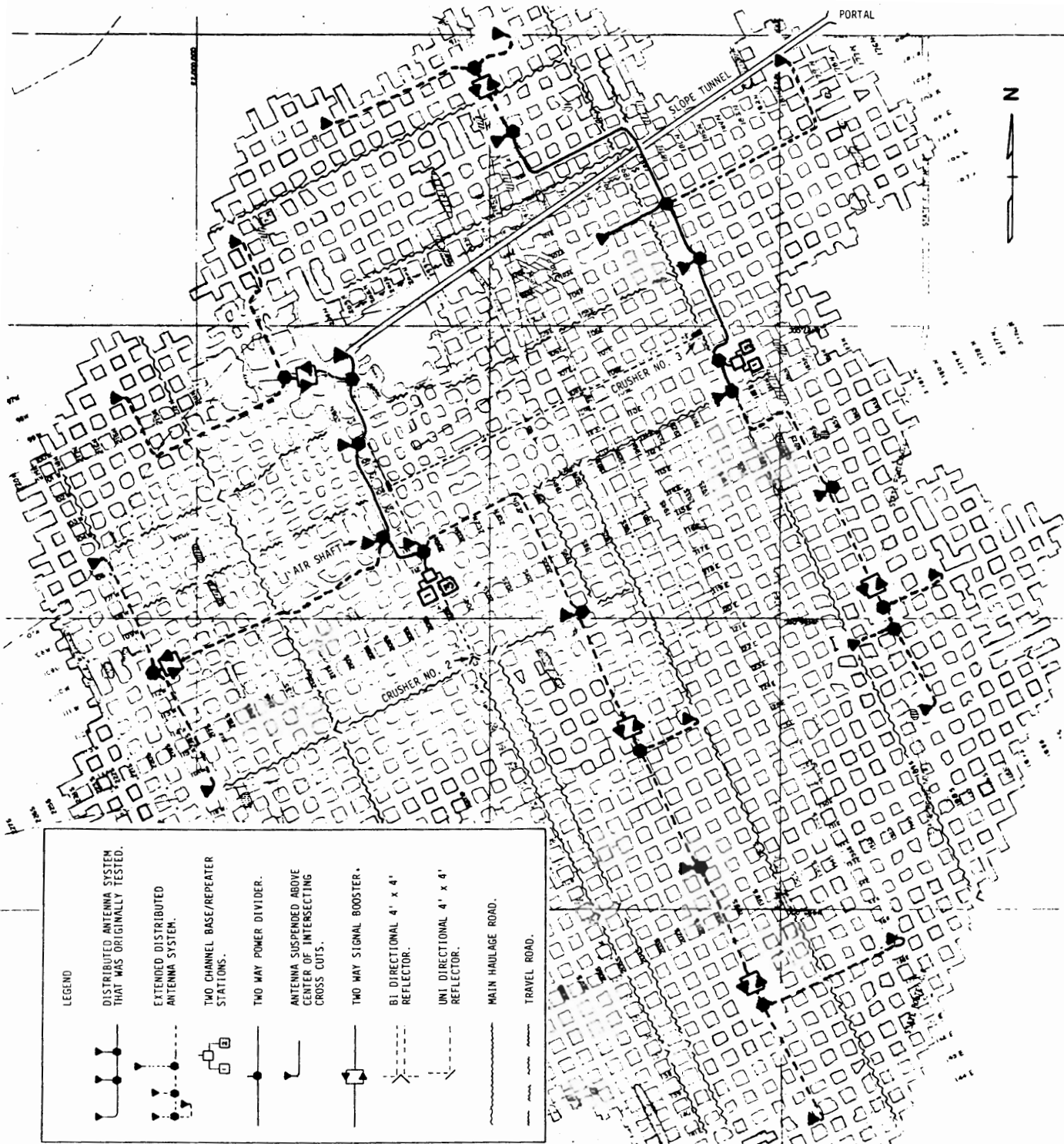
FIGURE 3.10. MAP OF BLACK RIVER MINE SHOWING EXTENDED ANTENNA SYSTEM AND LOCATIONS OF FUTURE SIGNAL BOOSTERS.
