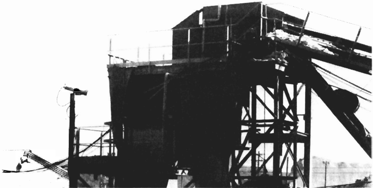
FIGURE 3.17. TV CAMERA VIEWING ROCK MOVEMENT AT THE TRANSITION OF CONVEYOR BELTS ABOVE THE MINE PORTAL.
