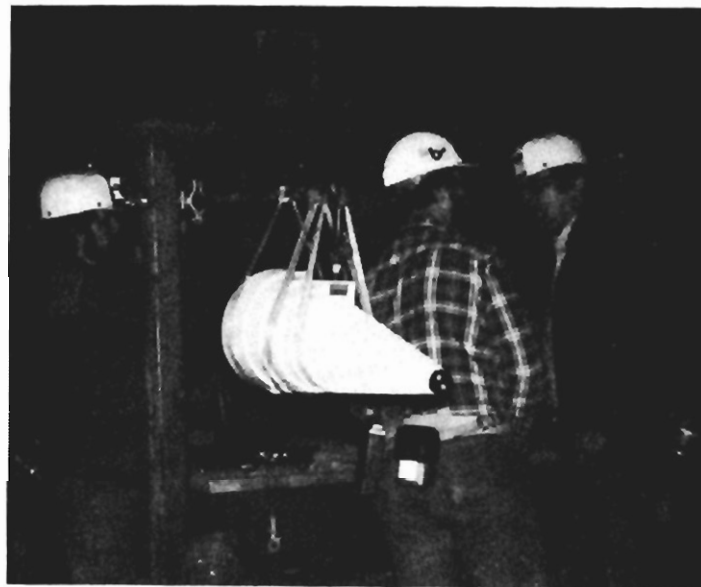
FIGURE 2.5. CIRCULARLY POLARIZED ANTENNA USED FOR SIGNAL STRENGTH MEASUREMENTS IN THE SLOPE TUNNEL.
