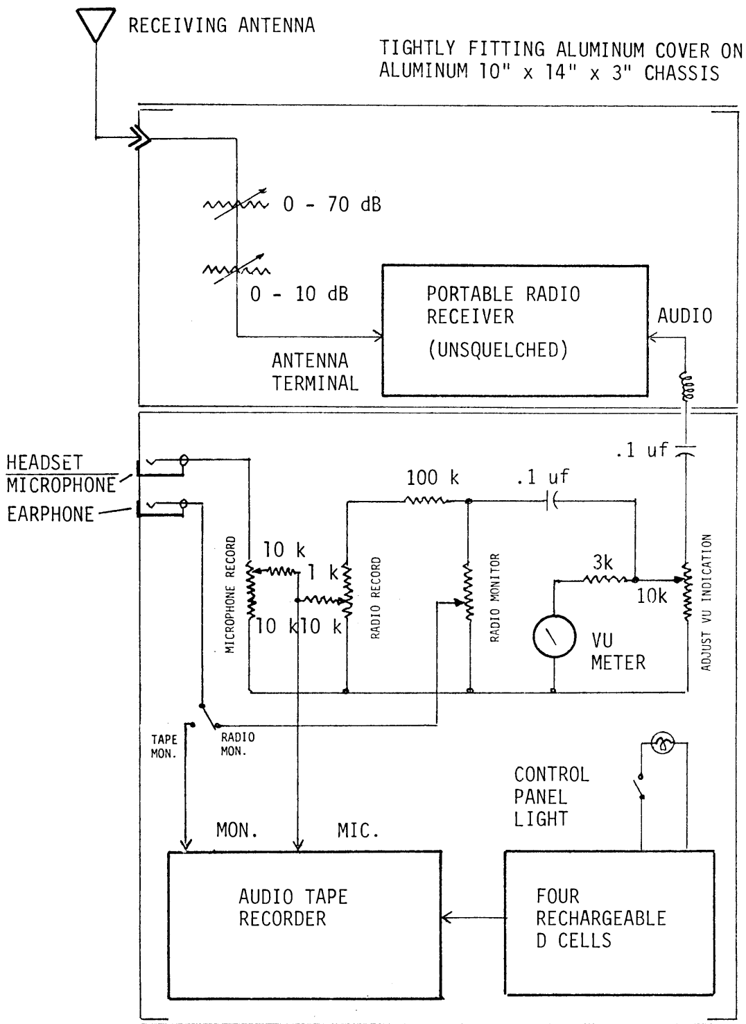
FIGURE 3.5. SCHEMATIC DIAGRAM OF SIGNAL MARGIN MEASURING EQUIPMENT
