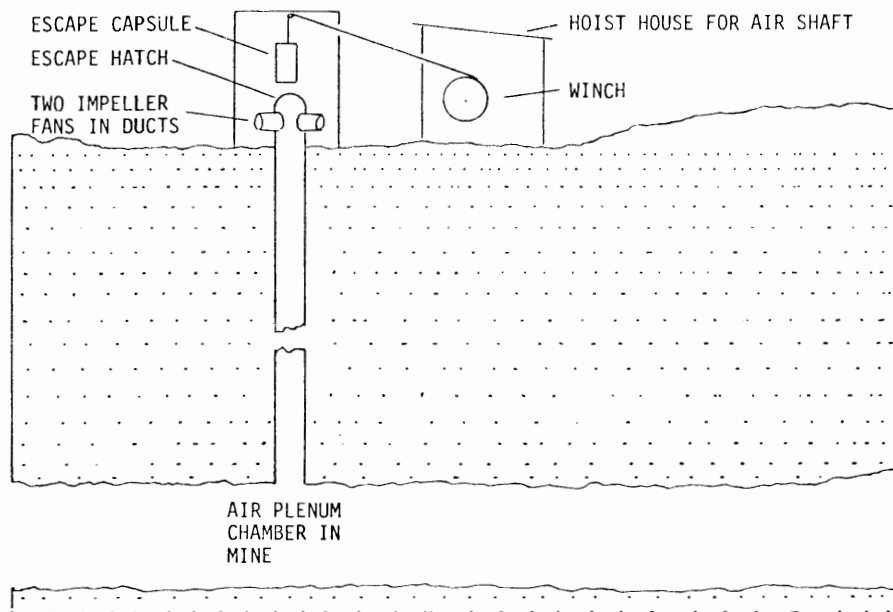
FIGURE 2.8 SKETCH OF AIR SHAFT USED AS EMERGENCY EXIT.
