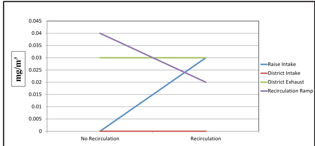
Respirable dust concentrations during normal and recirculation conditions.
