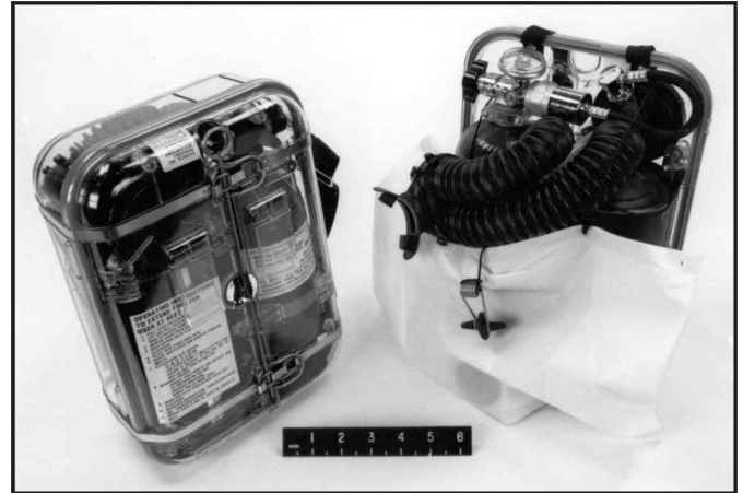
Figure 5.—Cased and uncased Ocenco EBA 6.5 self-rescuer.
