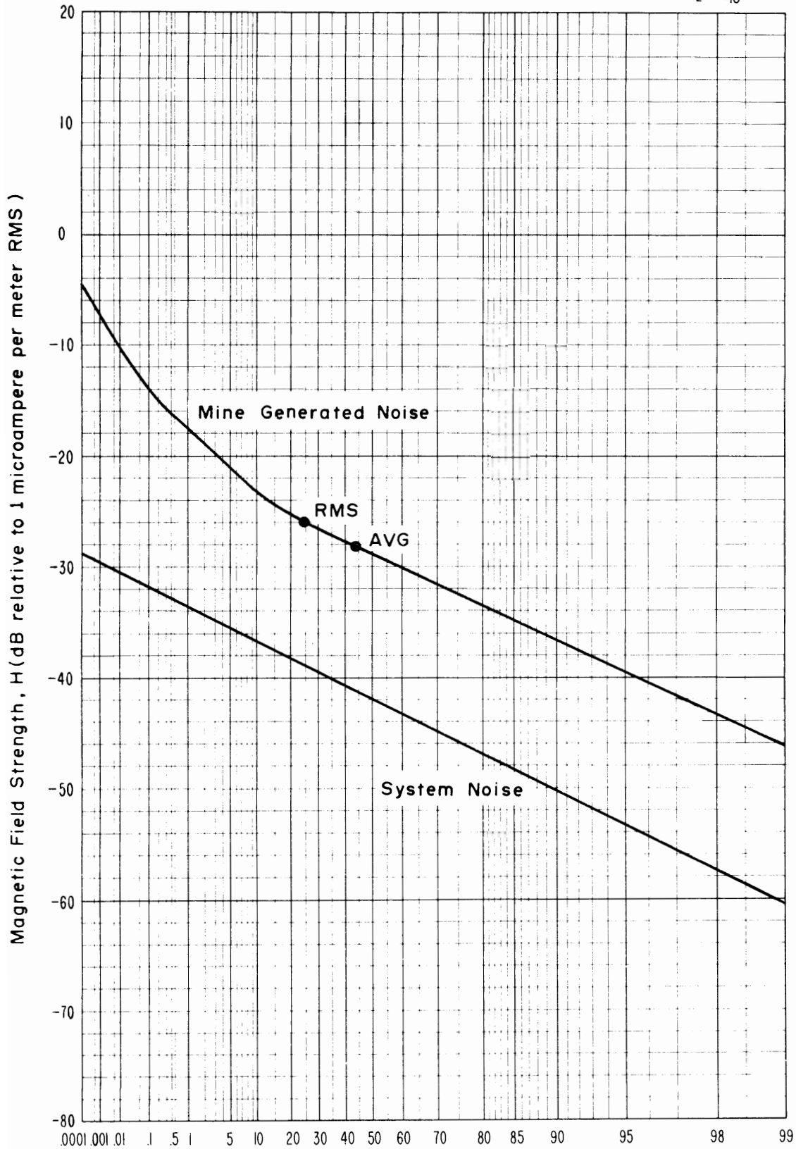
Figure 4-37 APD, 160 kHz, horizontal component E-W, 1.0 kHz predetection bandwidth, April 24, 1973, 4:15 p.m., shop office, Grace Mine.
