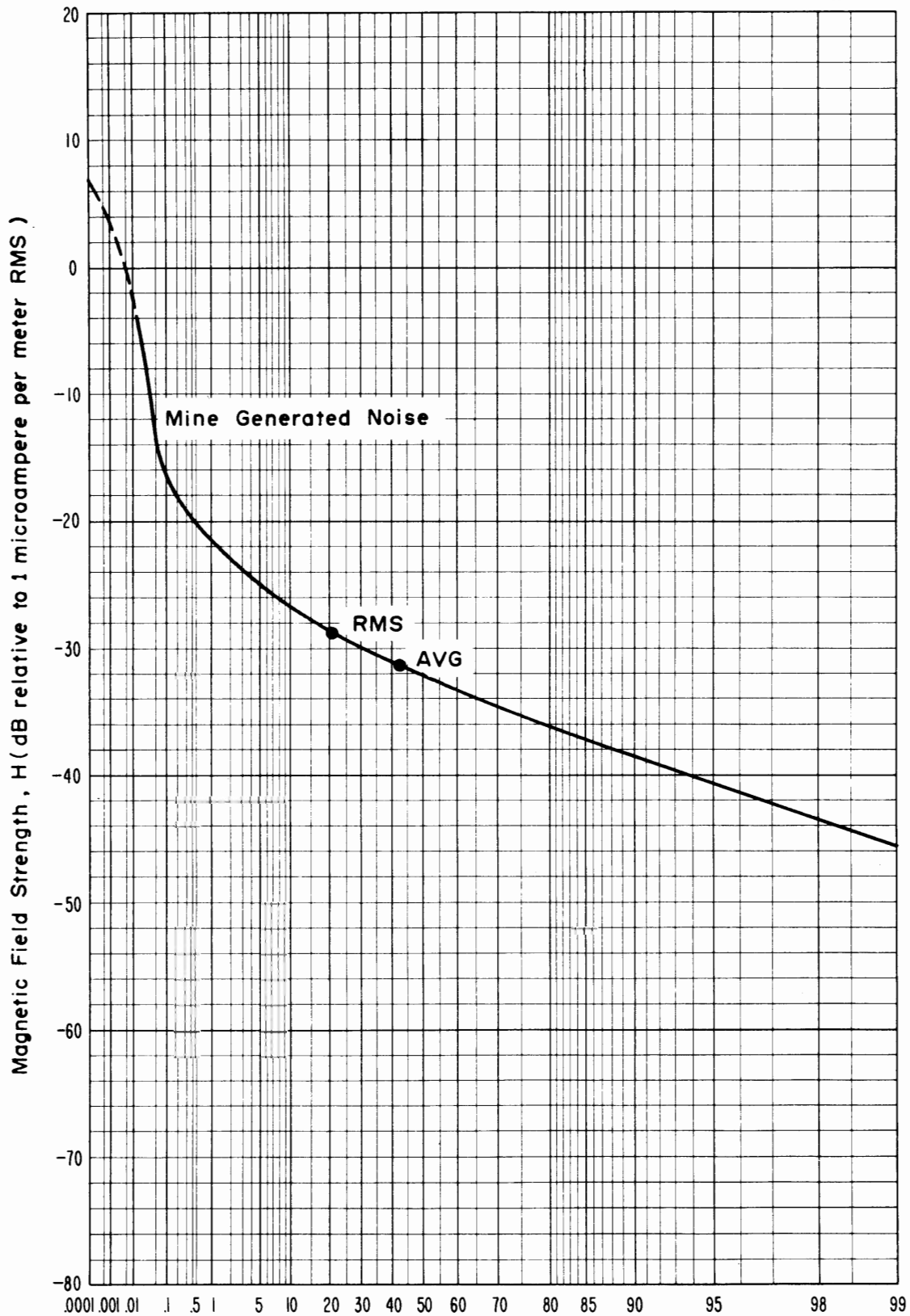
Percent of Time Ordinate is Exceeded Figure 4-36 APD, 130 kHz, horizontal component E-W, 1.0 kHz predetection bandwidth, April 24, 1973, 3:00 p.m., shop office, Grace Mine.
