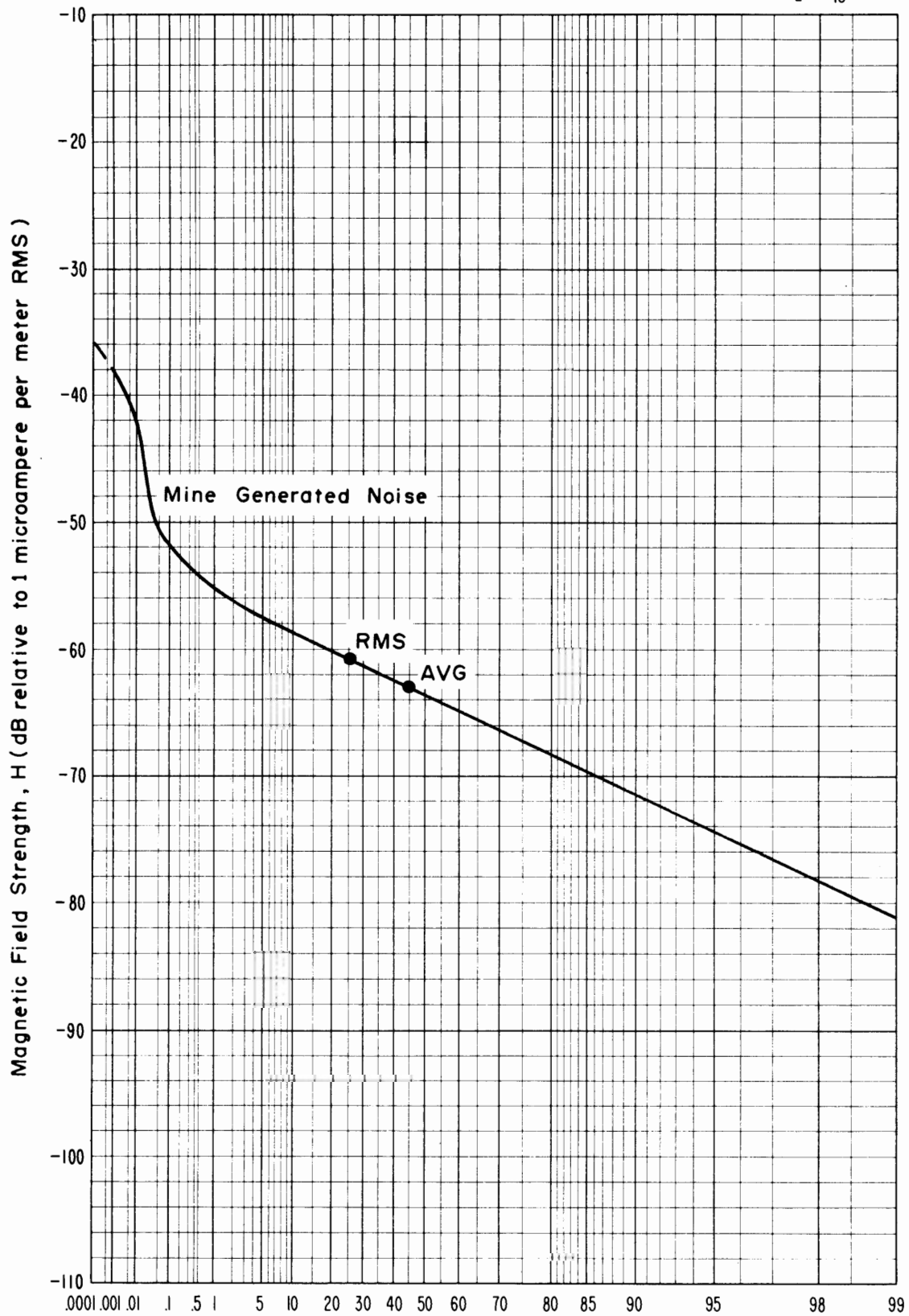
Figure 4-30 APD, 6 MHz, vertical component, 1.2 kHz predetection bandwidth, April 24, 1973, 4:45 p.m., shop office, Grace Mine.
