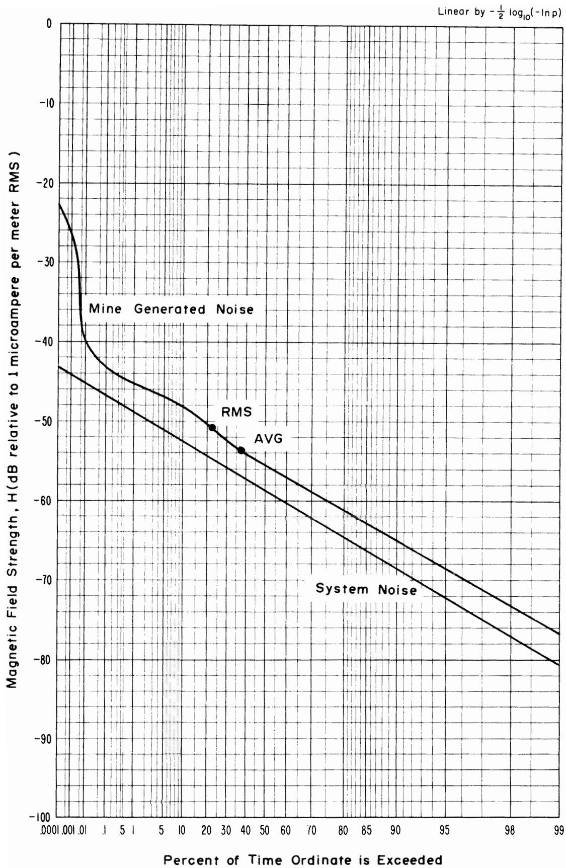
Figure 4-11 APD, 32 MHz, vertical component, 1.2 kHz predetection bandwidth, April 24, 1973, 12:40 p.m., development foreman office, Grace Mine.
