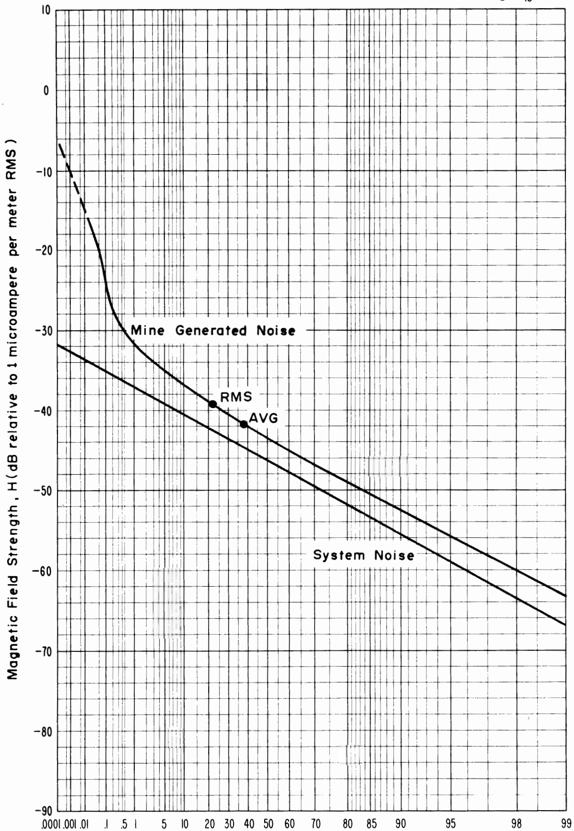
Percent of Time Ordinate is Exceeded Figure 4-38 APD, 250 kHz, horizontal component E-W, 1.2 kHz predetection bandwidth, April 24, 1973, 3:35 p.m., shop office, Grace Mine.
