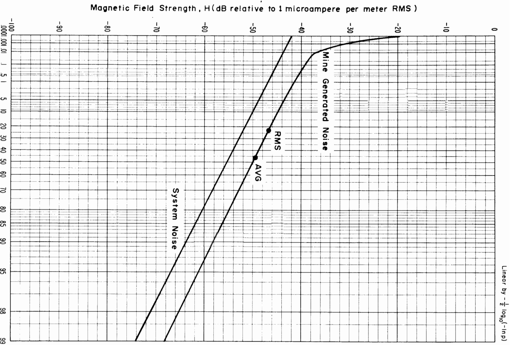
Figure 4-42 APD, 6 MHz, horizontal component E-W, 1.2 KHz predetection bandwidth, April 24, 1973, 4:15 p.m., shop office, Grace Mine.
