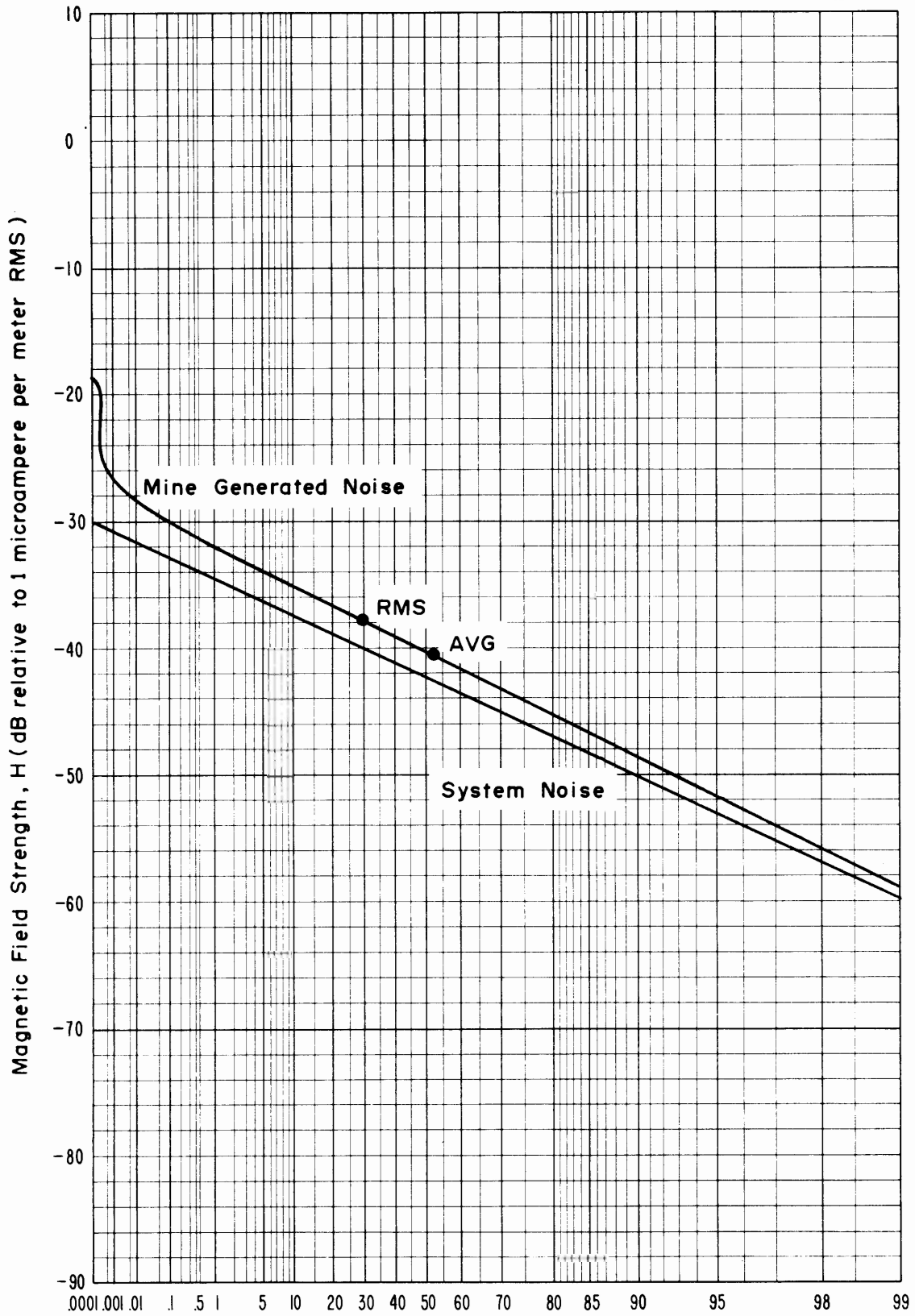
Figure 4-10 APD, 14 MHz, vertical component, 1.2 kHz predetection bandwidth, April 24, 1973, 12:10 p.m., development foreman office, Grace Mine.
