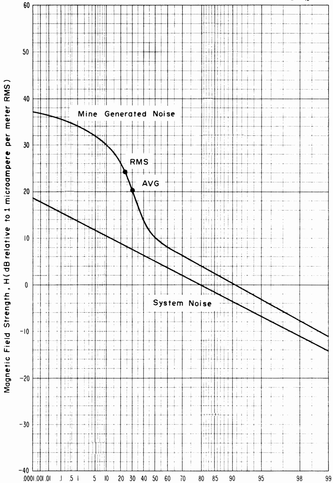
Percent of Time Ordinate is Exceeded Figure 4-12 APD, 10 kHz, vertical component, 1.0 kHz predetection bandwidth, April 24, 1973, 3:00 p.m., crusher substation, Grace Mine.
