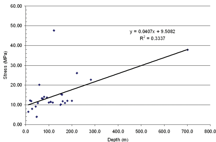
Figure 1—Maximum horizontal stress measurements in limestone and dolomite formations in the Eastern and Midwest US and Eastern Canada, showing a fitted straight line and equation
