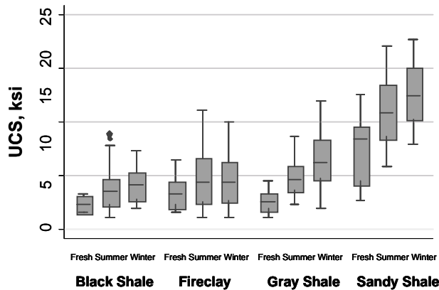
Figure 8. Graph showing PLT UCS values for the four clay rich rock types studied. In each case, the strengths were lowest when the cores were fresh, and highest during the winter when the rocks were driest. The middle line represents the median value, and the upper and lower hinges of the box represent the 75 th and 25 th percentiles of the data.
