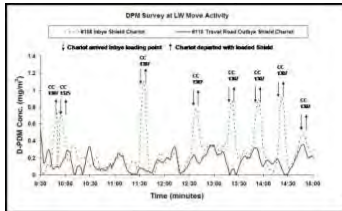
Figure 5: Diesel vehicle activities as measured by D-PDM
