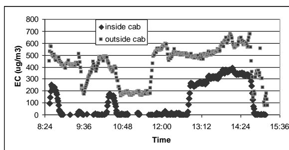
Figure 4: Interior and exterior cab EC concentration using a 5-minute running average during test 1.
