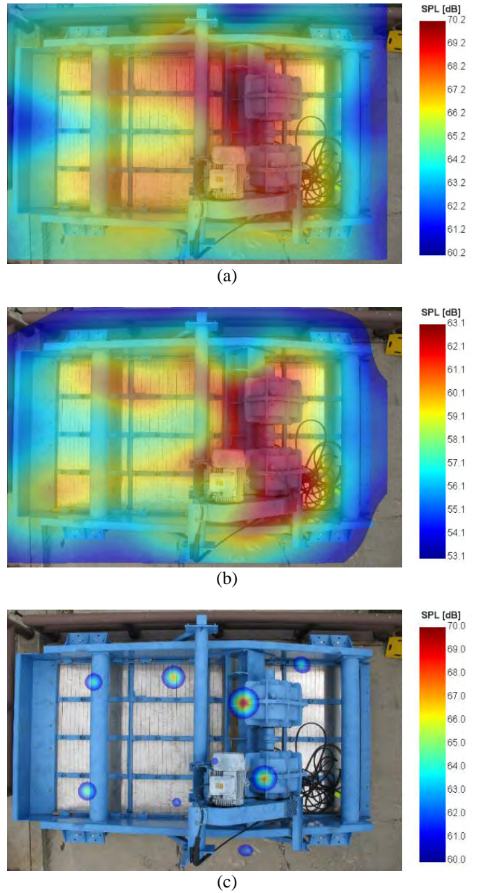
Figure 5. Comparison of acoustic maps at 315 Hz obtained with: a) CB, b) RCB, and c) CLEAN-SC.
