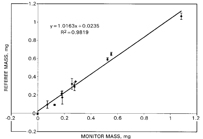
Figure 3.—Mass comparison between referee samplers and the continuous respirable dust monitor.
