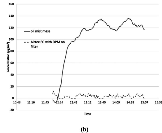
Fig. 8 Airtec measurement in the presence of oil mist in the test chamber with (b) and without (a) DPM collected on the filter.
