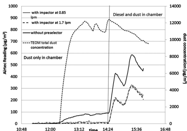
Fig. 4 The concentration of total dust from a metal mine in the test chamber, with and without DPM, and the measurement of the Airtecs at the same time.
