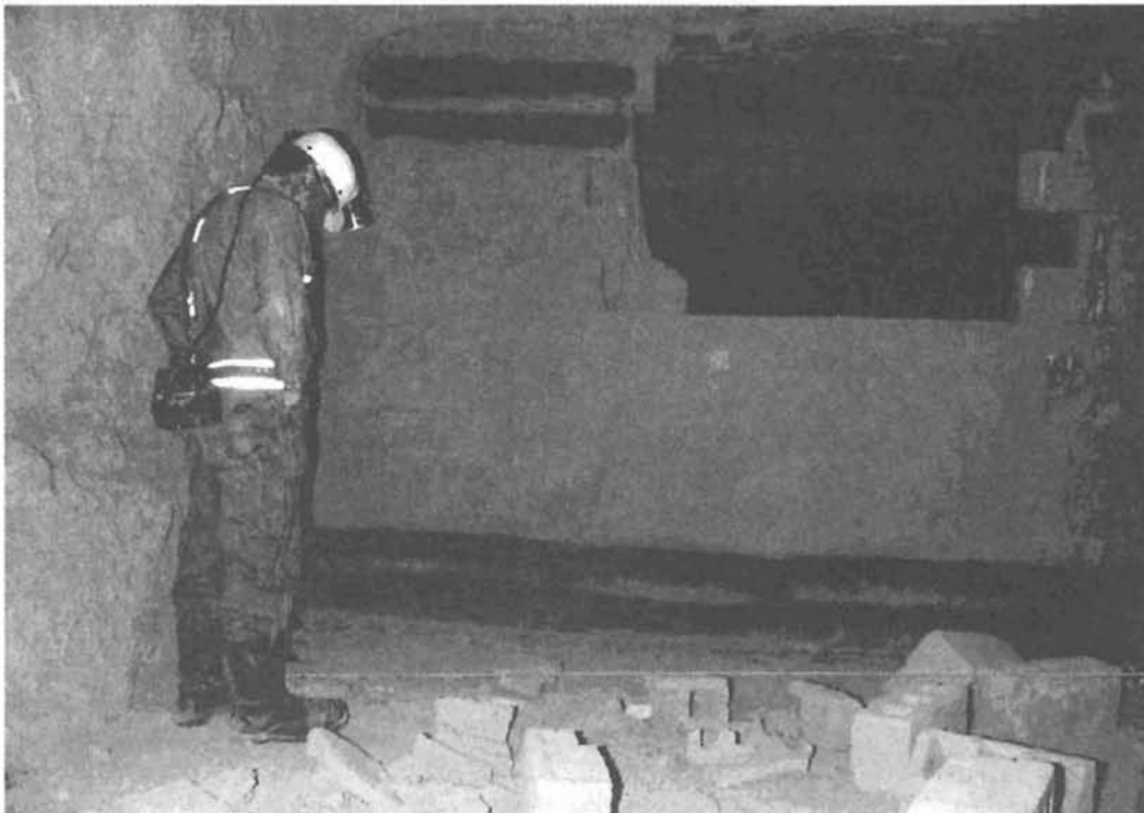
Figure 2. Ventilation stopping partially destroyed by explosion pressure.
