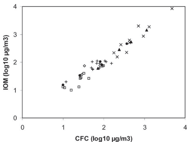
Fig. 1 Comparison of filter only analyses for lead (Pb) from side by side IOM and CFC samplers ( n = 51 ; y = 1.02x , r^2 = 0.93 ). \times ← lead acid battery recycler, \diamond bronze foundry, \blacktriangle lead ore processing mill, + copper ore smelter, \square nickel chromium recycler, \bullet solder manufacturer. Also published in ref. 12.
