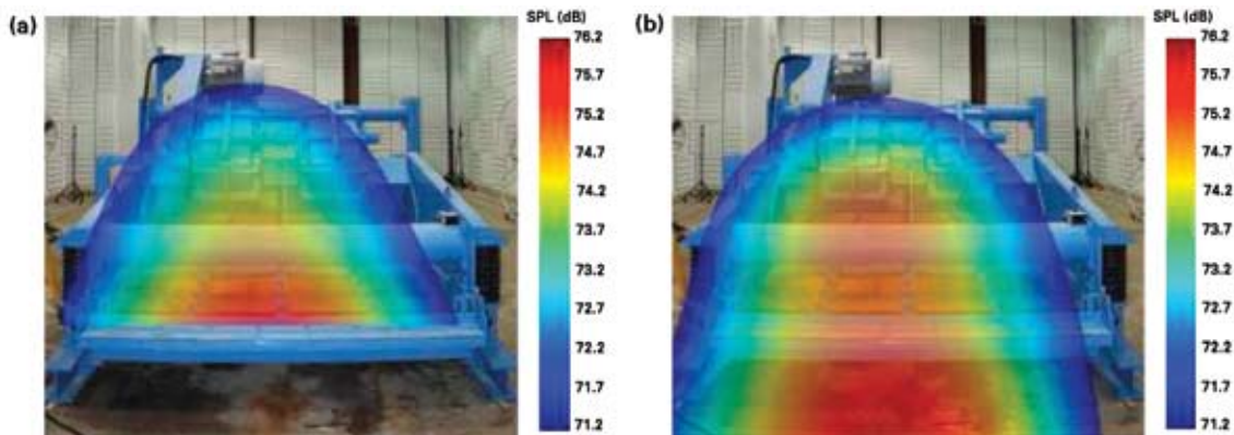
Acoustic maps at 250 Hz. Scanning planes at (a) eccentrics shaft and (b) discharge end.
