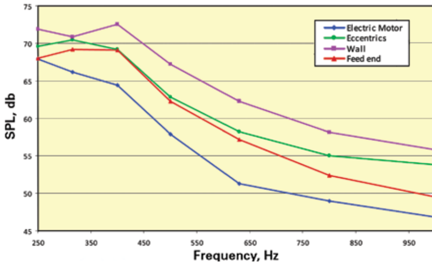
Integrated spectra. Array on electric motor side.
