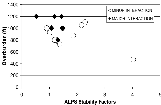
Figure 4. Relationship between degree of interaction and the Harris No. 1 ALPS stability factors and overburden.
