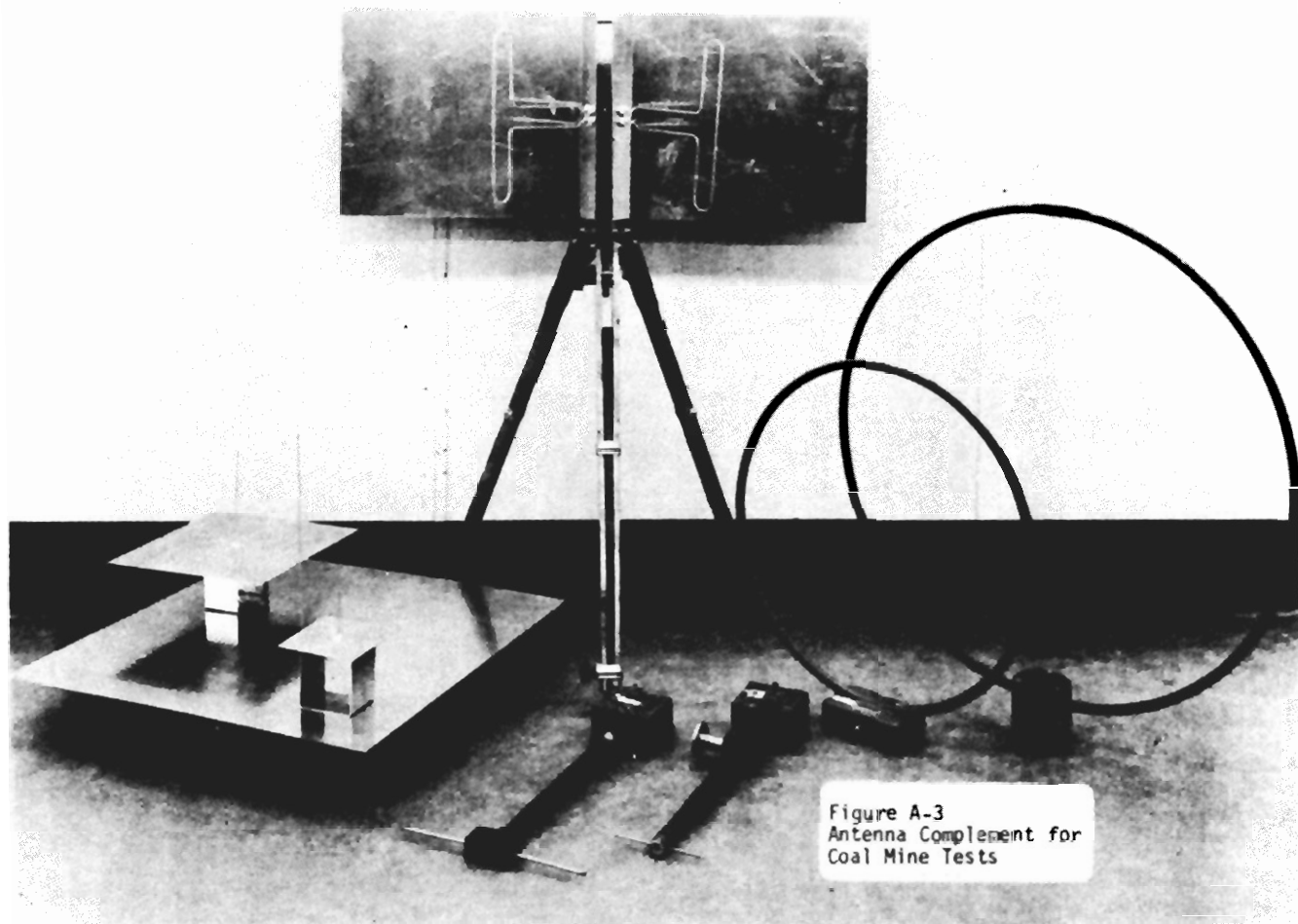
Figure A-3. Antenna Complement for Coal Mine Tests.
