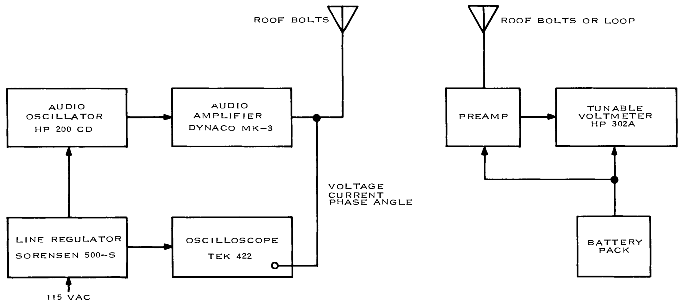
Figure A-2. VLF Test Setup.
