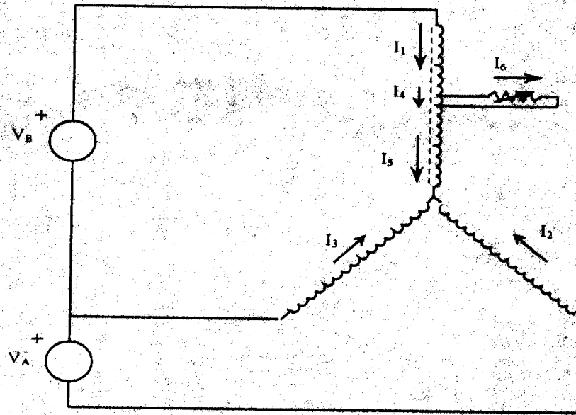
Fig. 3. Network diagram of the deteriorating motor model stator.
