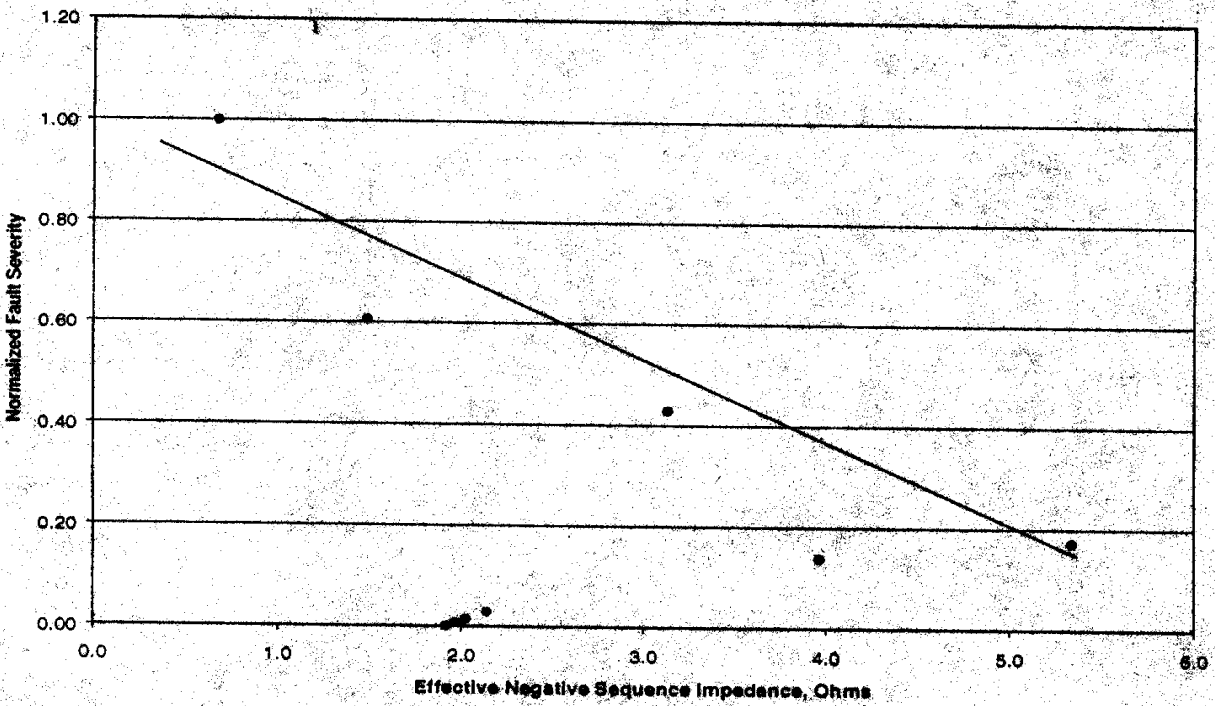
Figure 4. Effective negative-sequence impedance versus fault severity.
