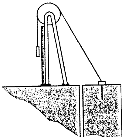
Figure 3 – Wire extensometer
