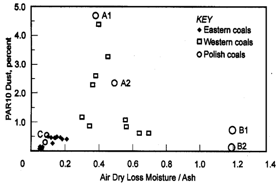
Figure 3. Relationship between PAR10 dust and the ratio of air dry loss moisture \div ash content.
