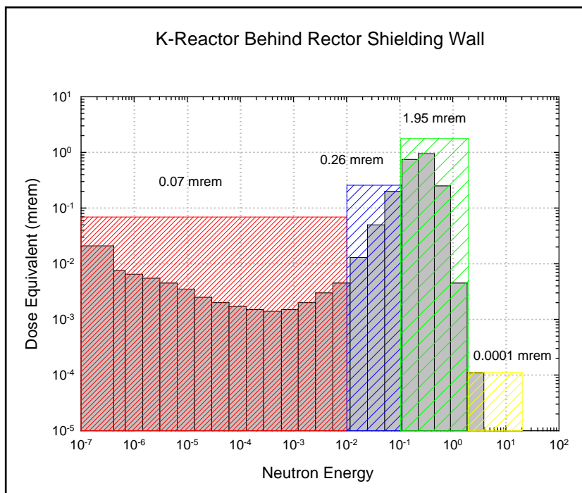
Figure 5.3.4.2-3. Neutron energy spectra recorded behind the K-Reactor shield door with neutron energy groups overlay.
