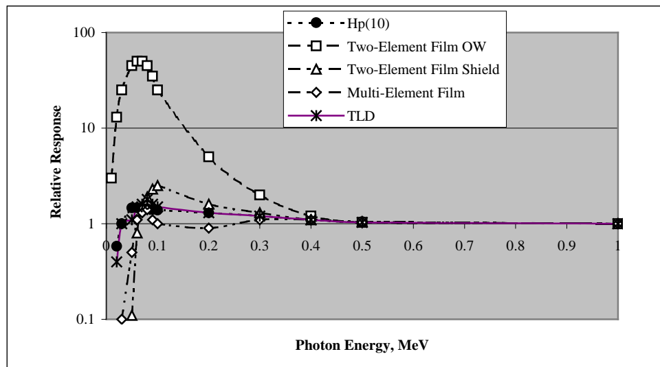
Figure 5.3.2.1-1. Estimated SRS dosimeter photon response characteristics.
