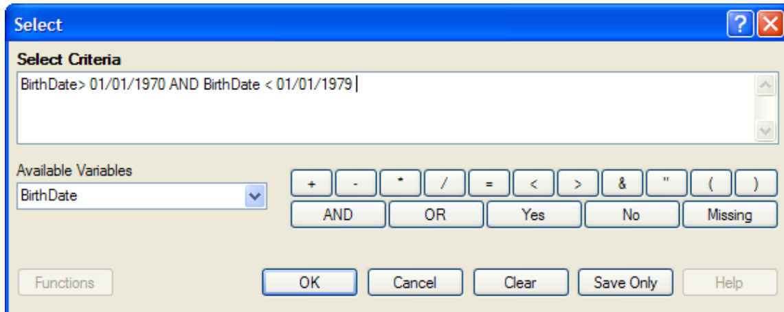
Figure 9.22: Select Dialog Box
