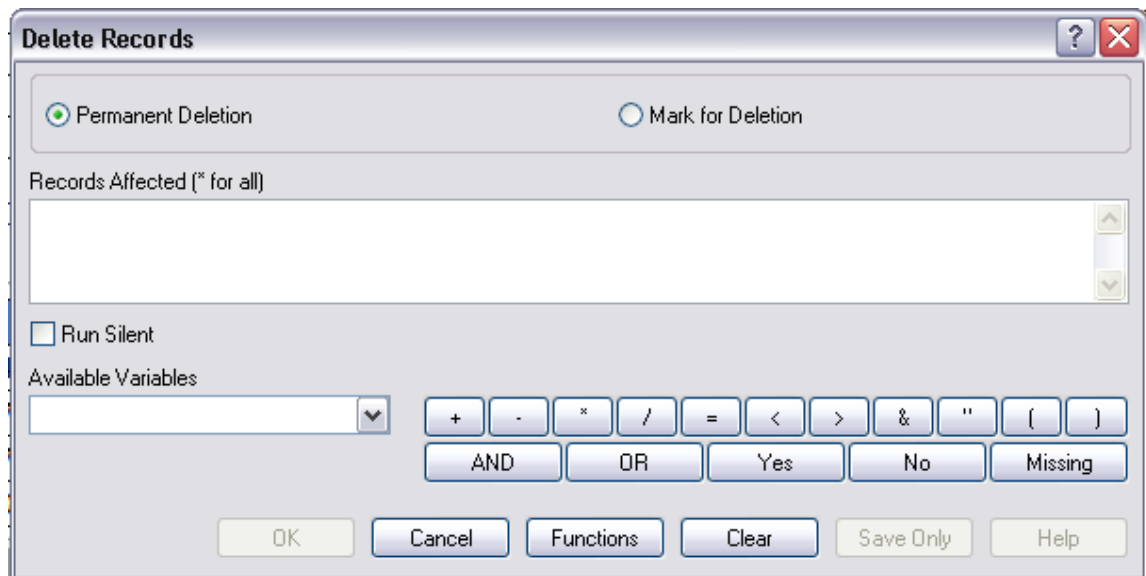
Figure 9.11: Delete Records Dialog Box
