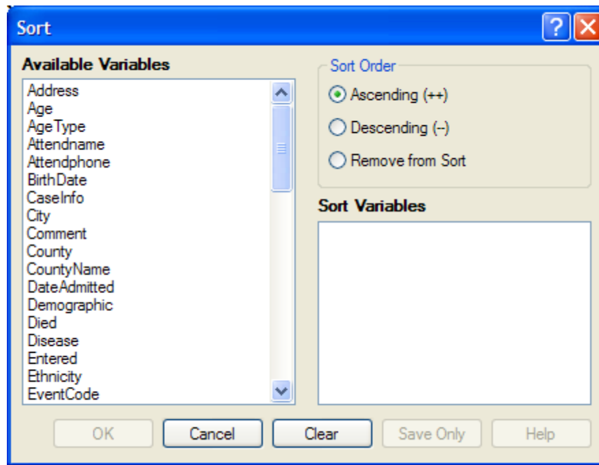
Figure 9.25: Sort Command Dialog Box
